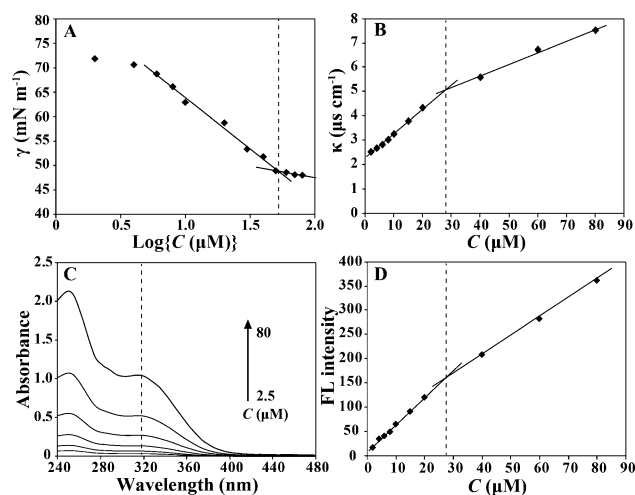
Figure 2. A) Plot of surface tension versus \log (concentration) for TPE-SDS. B) Plot of conductivity versus the concentration of TPE-SDS. C) Absorption spectra of TPE-SDS at different concentrations. D) Plot of fluorescence intensity at 490 nm versus the corresponding TPE-SDS concentration.
